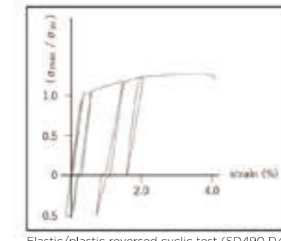
Elastic/plastic reversed cyclic test (SD490 D41)
