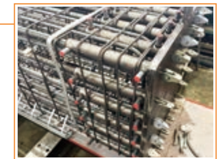
Precast column production
